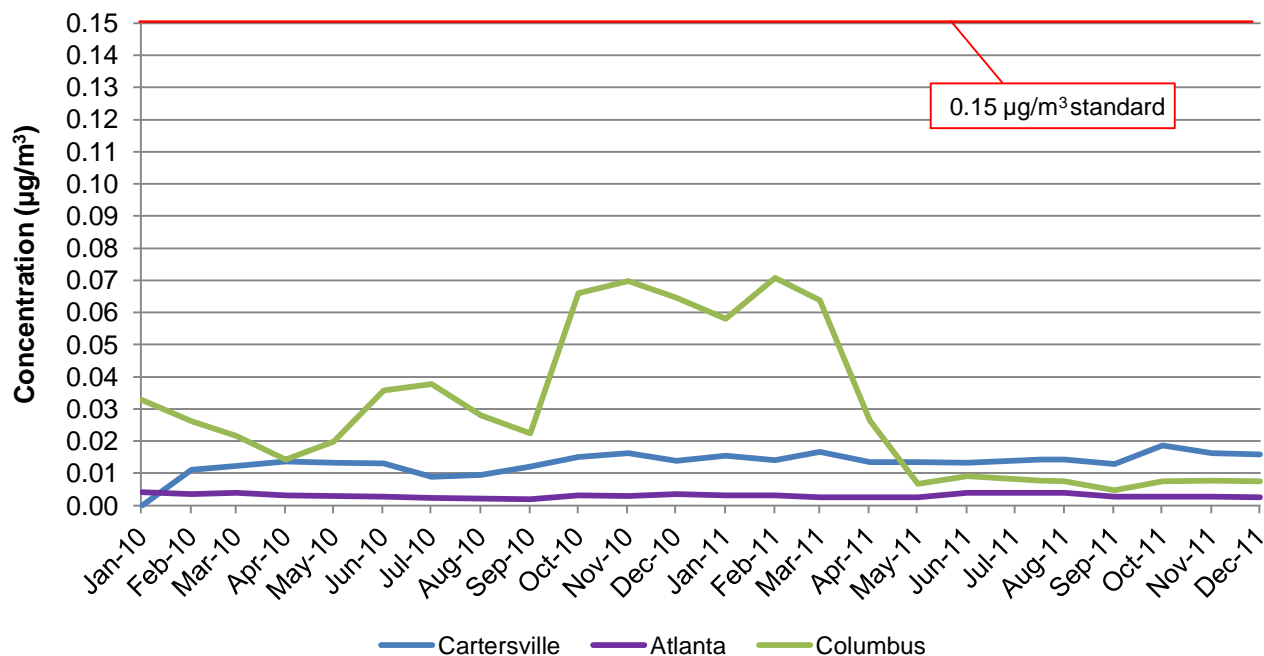
Figure 32: Three-Month Rolling Averages of Lead, 2010-2011
