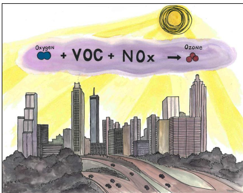
Figure 19: Ozone Formation Process
