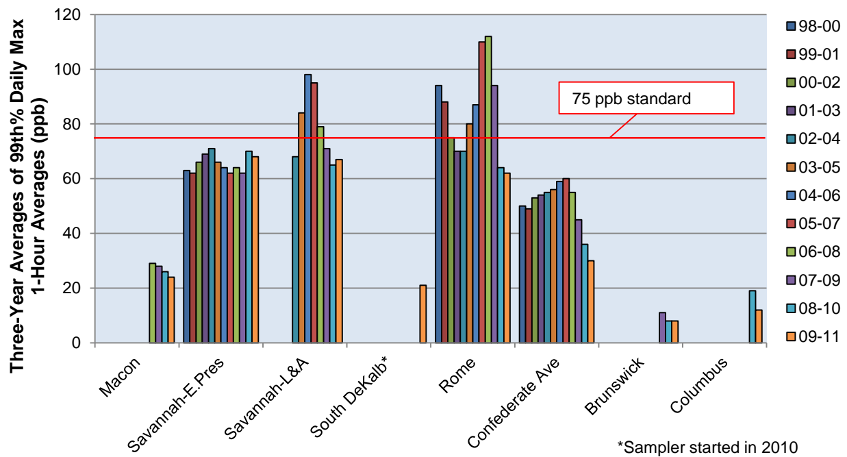
Figure 16: SO 2 1-Hour Design Values, 2000-2011
