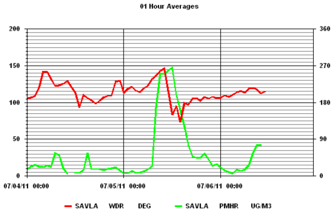
Figure 84: Wind Direction and Continuous PM 2.5 at Savannah L&A Site on July 5, 2011
