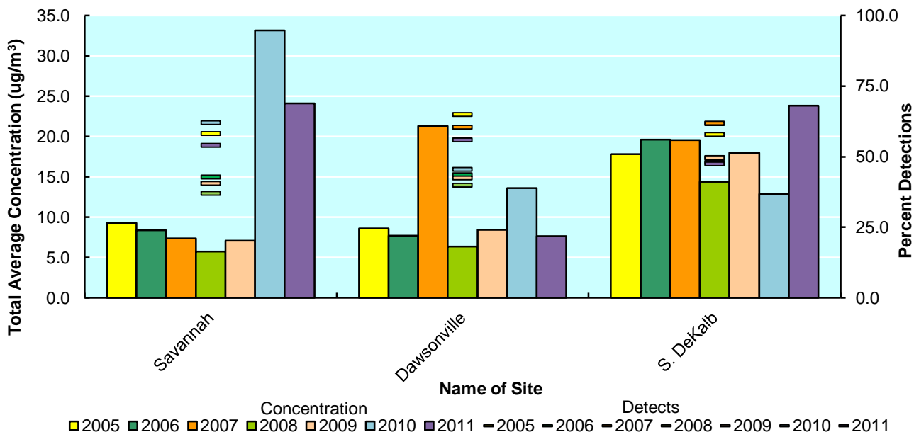
Figure 57: Average 24-Hour Carbonyls Concentration and Number of Detects, by Site, 2005-2011
