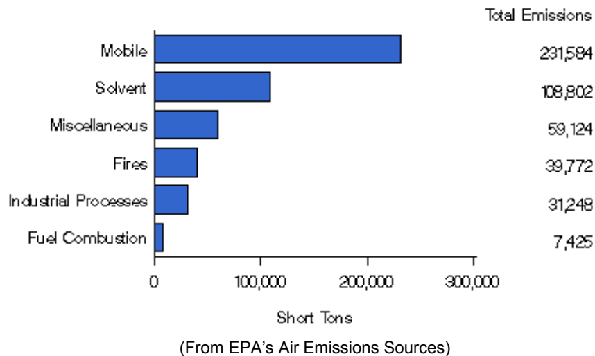
Figure 20: Common Sources of Volatile Organic Compounds (VOCs) in Georgia in 2008
