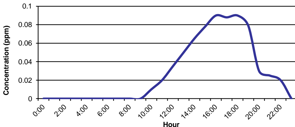
Figure 18: Typical Urban 1-Hour Ozone Diurnal Pattern
