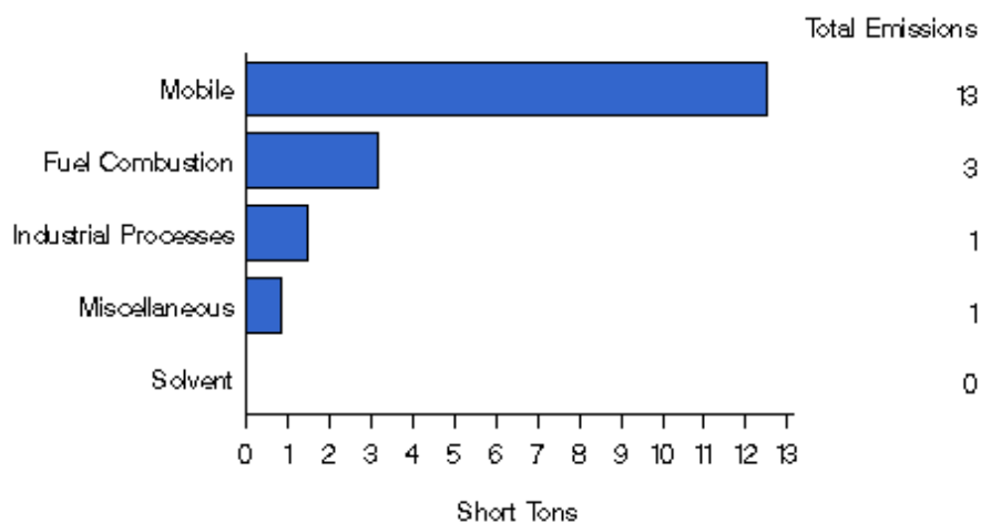
Figure 29: Common Sources of Lead in Georgia in 2008
