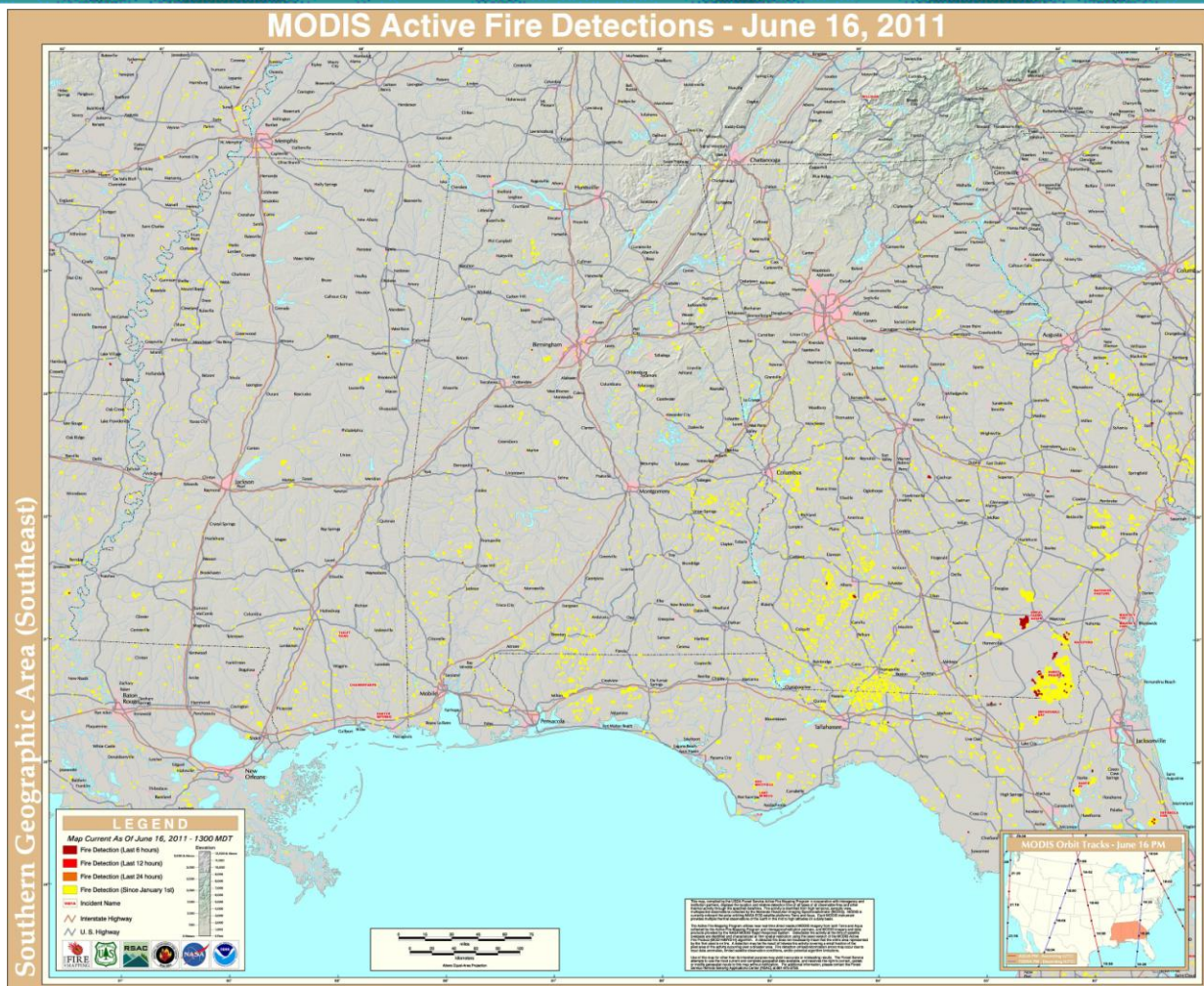
Figure 81: MODIS Locations of Fires on June 16, 2011
