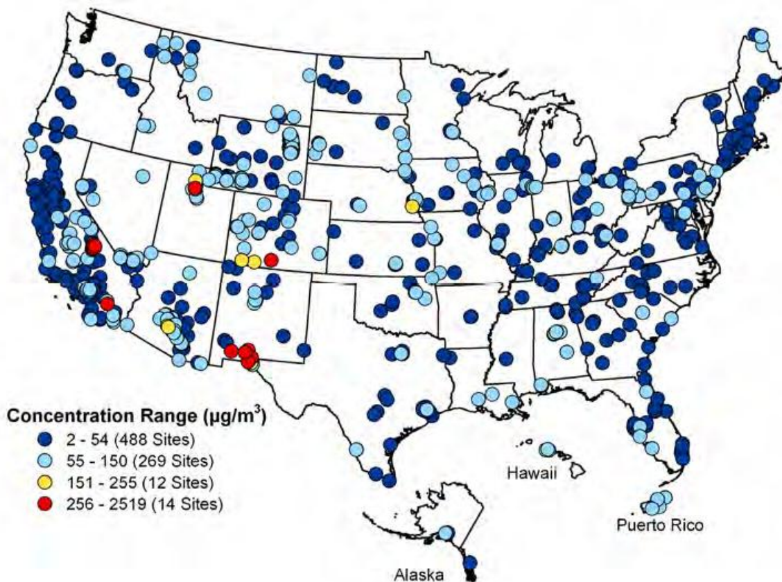
Figure 38: PM 10 Second Maximum 24-Hour Concentrations (µg/m 3 ), 2010
