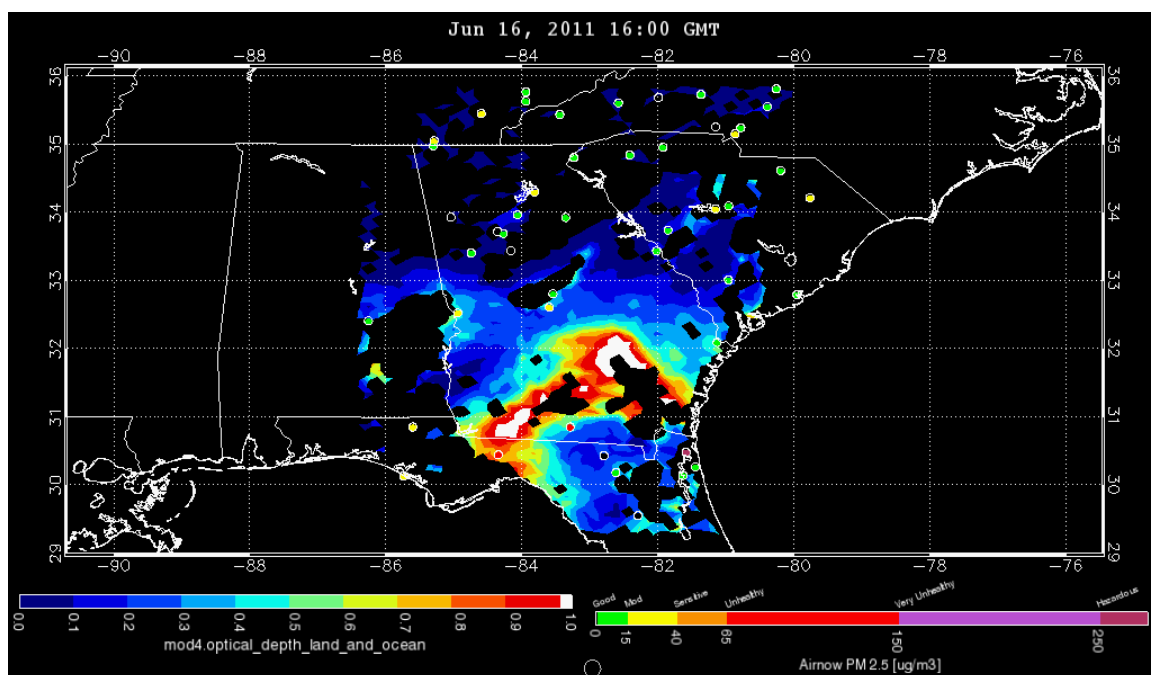
Figure 82: Aerosol Optical Depth with MODIS AOD Terra Imagery, June 16, 2011
