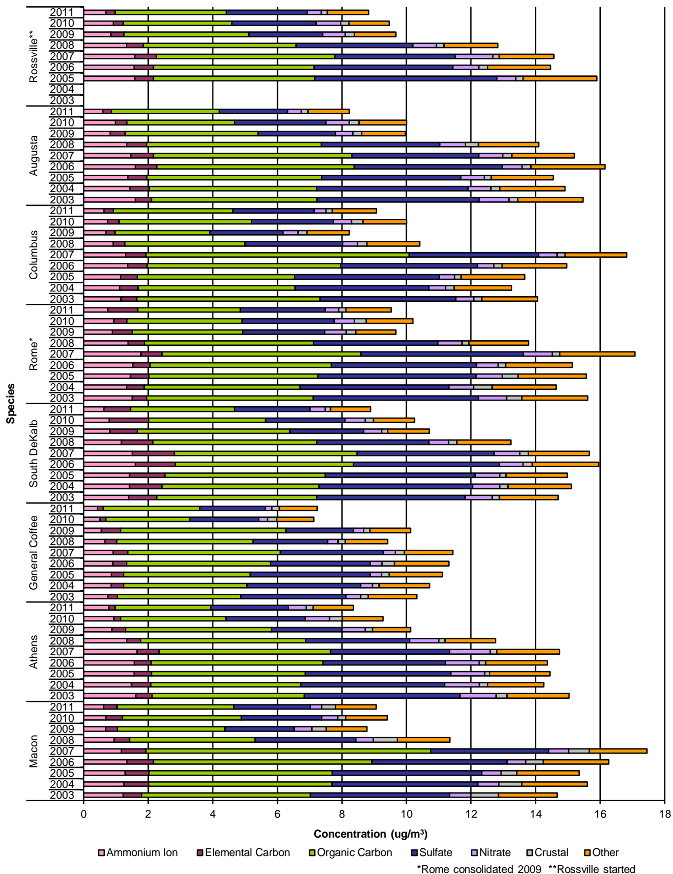
Figure 48: PM 2.5 Speciation, by Site, 2003-2011
