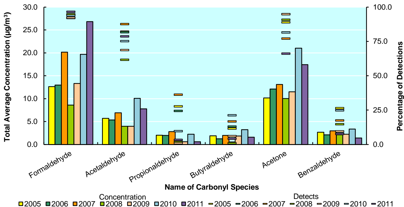
Figure 58: Average 24-Hour Carbonyls Concentration vs. Number of Detects, by Species, 2005-2011
