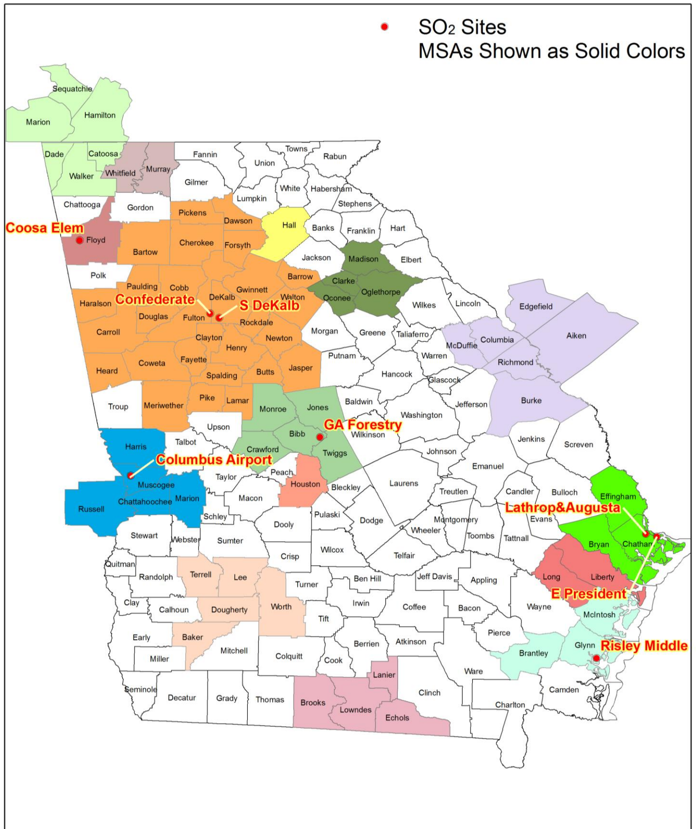
Figure 17: Sulfur Dioxide Monitoring Site Map
