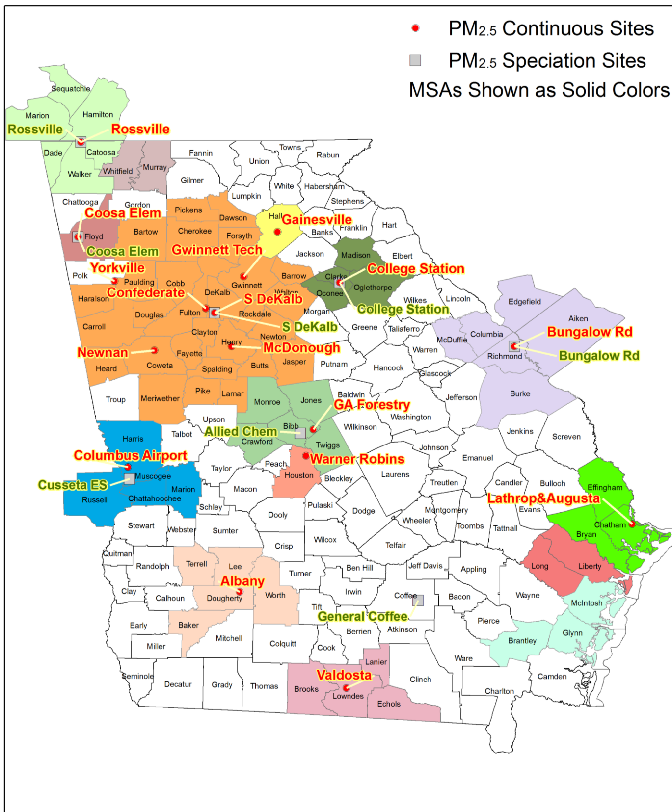
Figure 42: PM 2.5 Continuous and Speciation Monitoring Site Map
