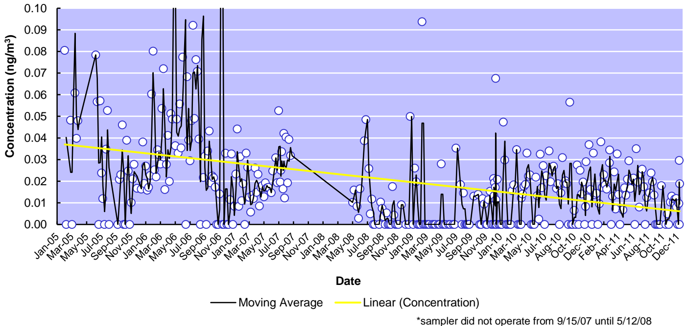
Figure 64: Hexavalent Chromium at South DeKalb
