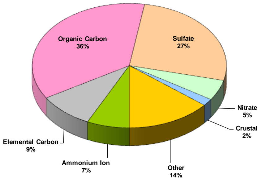
Particle Speciation- Atlanta 2011
