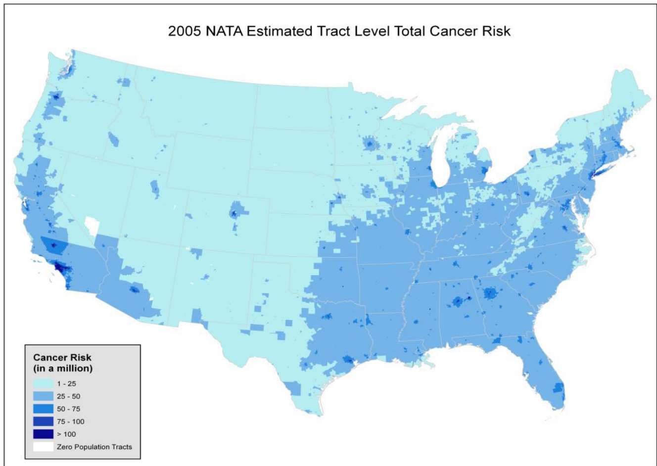
Figure 87: Estimated Tract-Level Cancer Risk from the 2005 National Air Toxics Assessment
