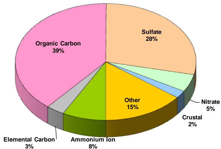
Particle Speciation - Rossville 2011
