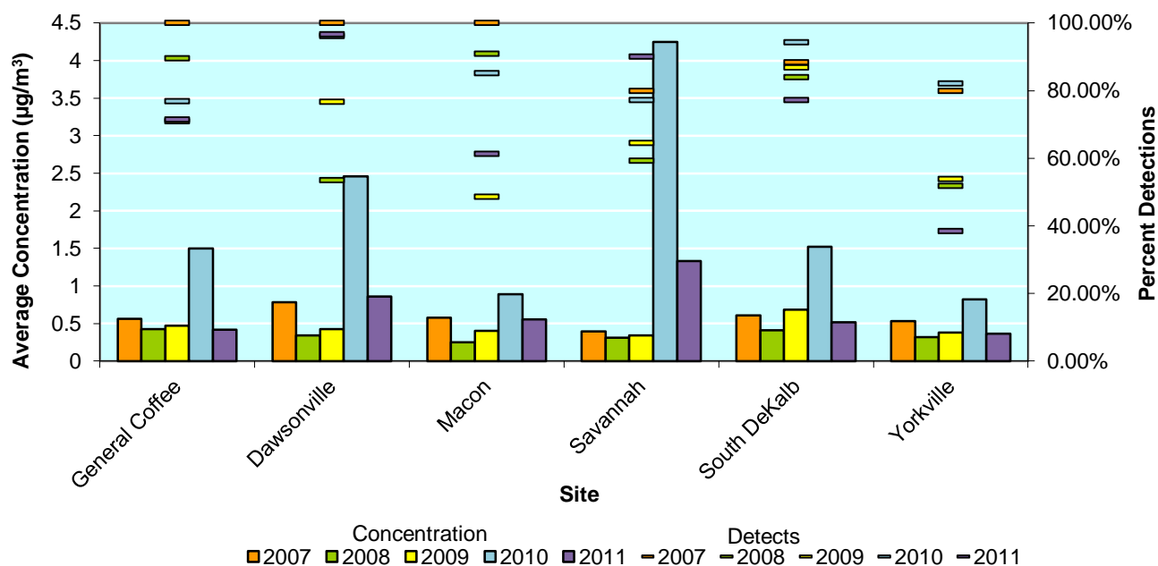
Figure 59: Acrolein Concentrations and Percent Detections, 2007- 2011
