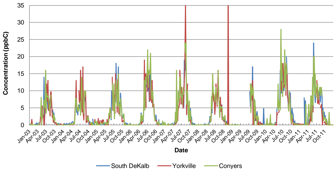
Figure 51: Isoprene Yearly Profile, 2003-2011
