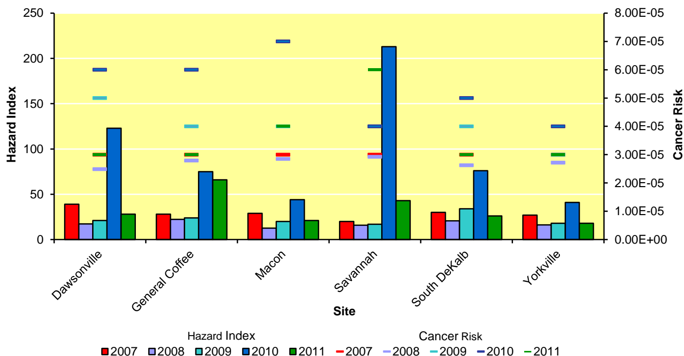
Figure 86: Aggregate Cancer Risk and Hazard Index by Site for 2007-2011
