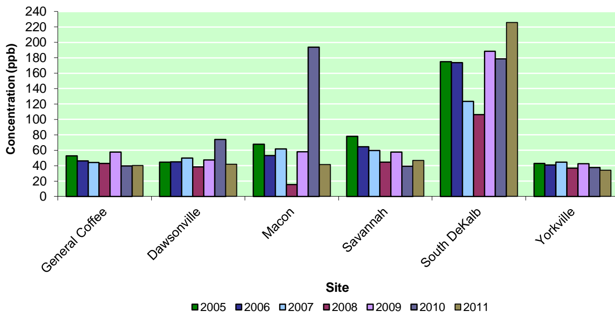
Figure 67: Total Volatile Organic Compound Loading all Species, by Site, 2005-2011
