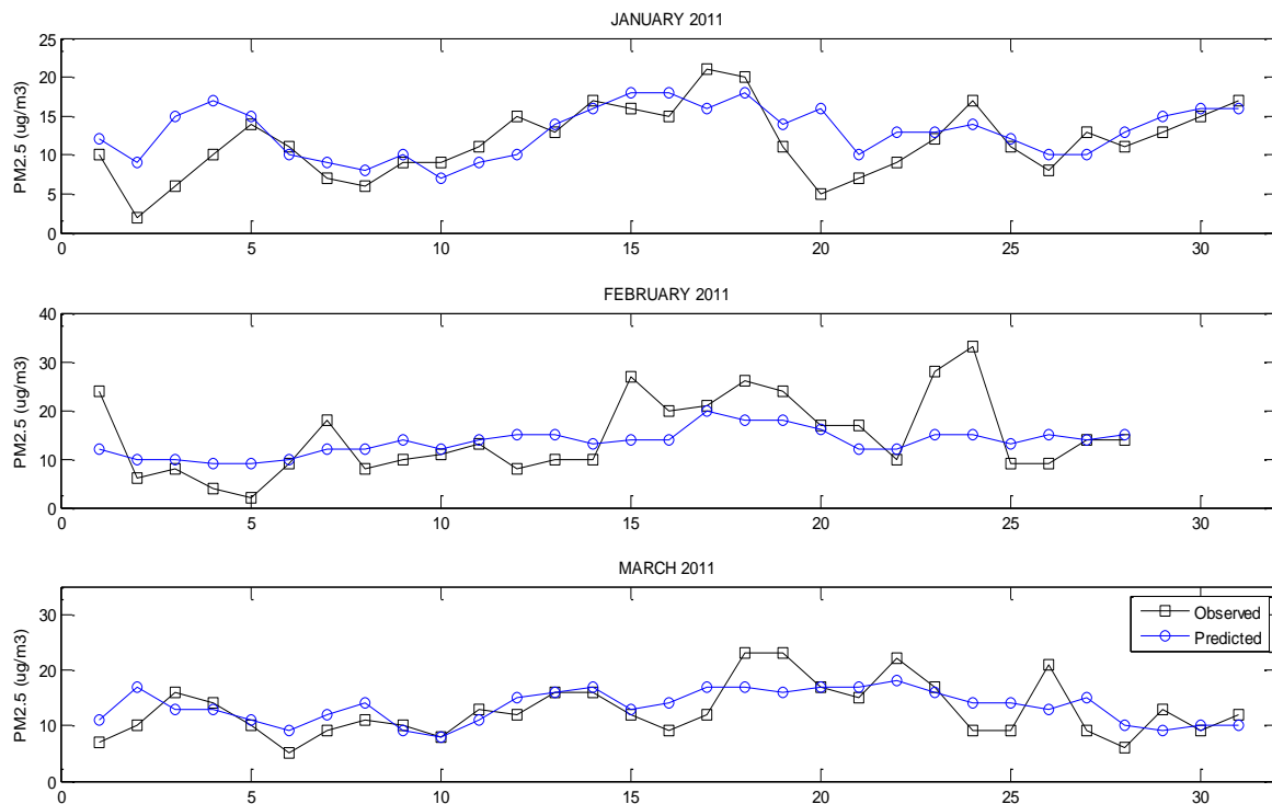
Figure 75: Monthly Time Series of PM_{2.5} Predictions and Observations for Metro Atlanta During 2011 (January-March)
