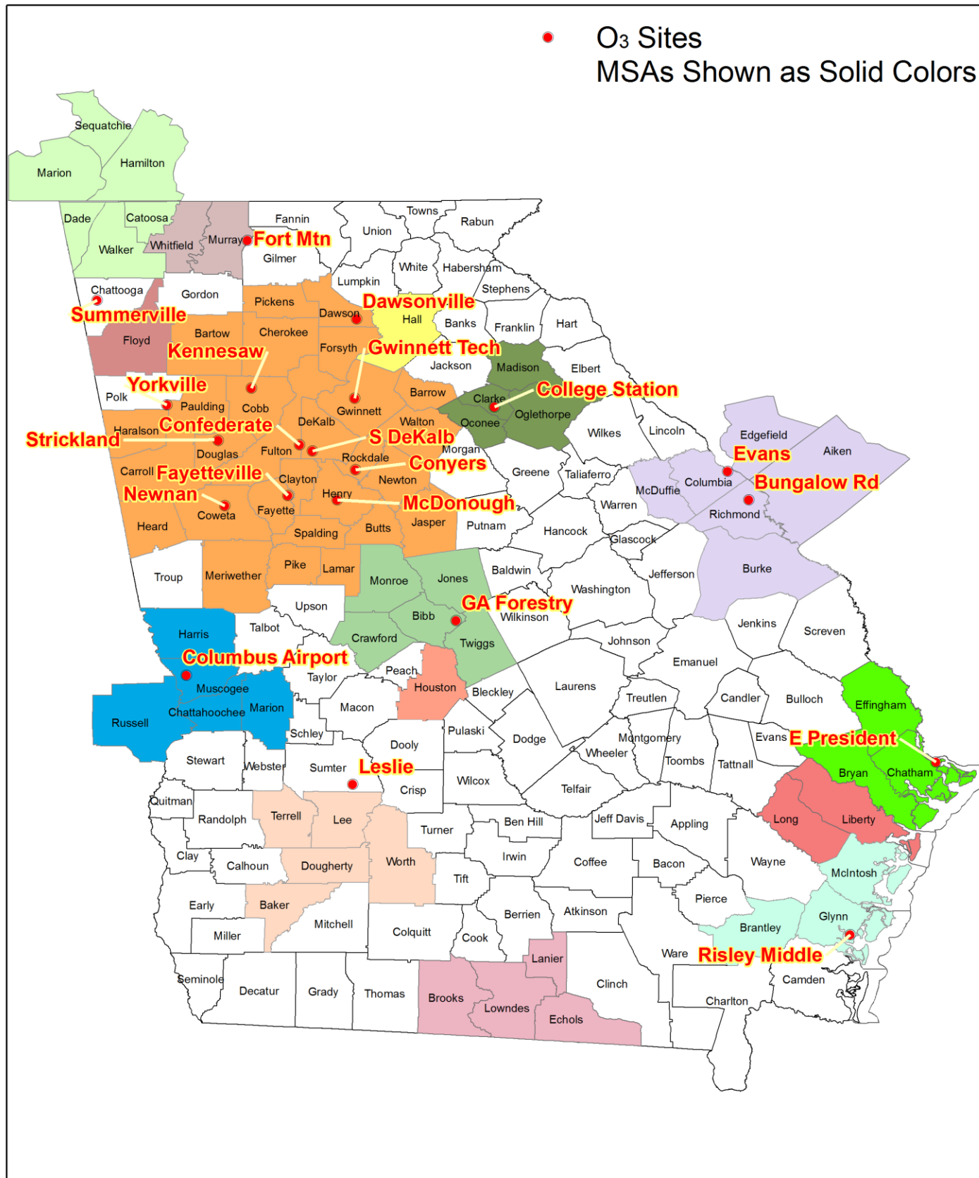
Figure 22: Ozone Monitoring Site Map
